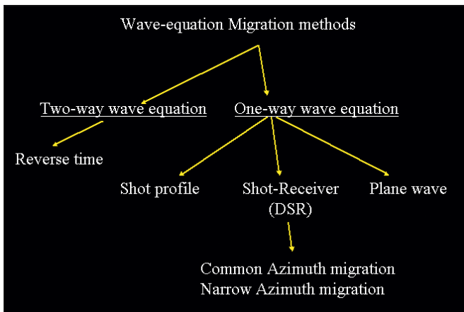
Figure 2. Alternative implementations of wave equation migration.
