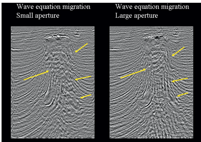
Figure 3. Migration aperture comparison. Note the recovery of ultra-steep dips when full aperture is invoked.
