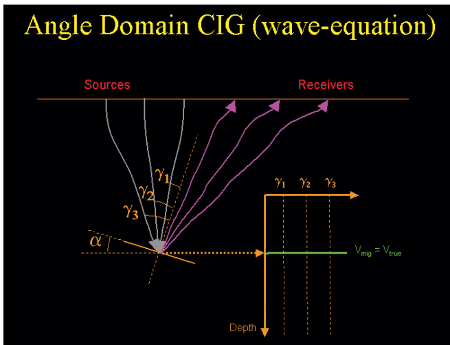
Figure 4. Gather energy is organized by reflection angle.
