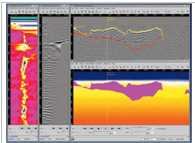
Figure 5. Interactive graphical aid for rapid model QC/validation showing angle gather with semblance.
