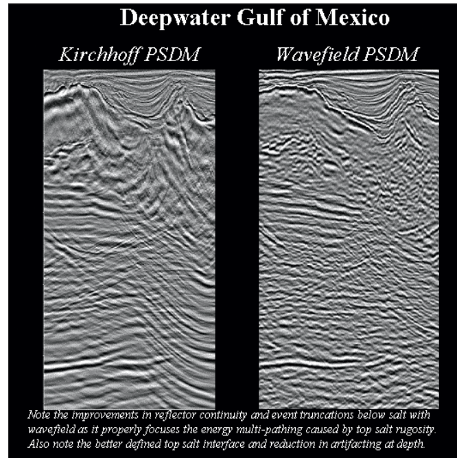
Figure 1. Kirchhoff versus wave equation: impact of strong top salt rugosity on below salt sedimentary interfaces.
