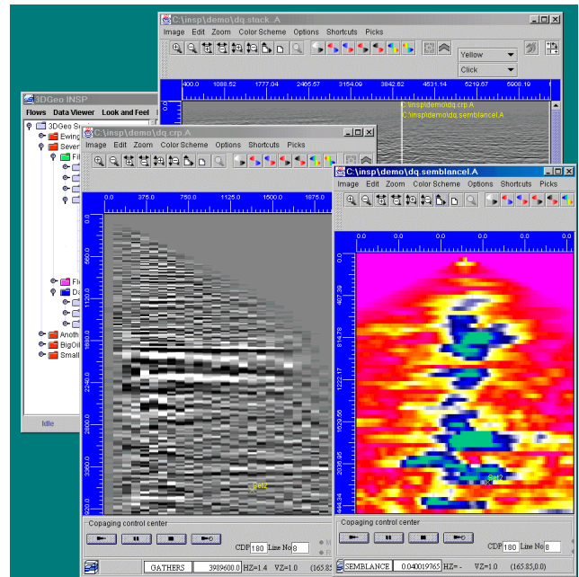
Fig. 3 INSP allows many data sets to be viewed concurrently over the Internet, allowing a remote user to QC processing jobs, interpret results, build velocity models, and perform processing tasks such as picking or editing.
